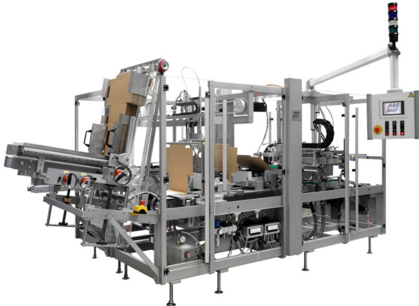
Abb. 2 B&B-MAF Combimatic
